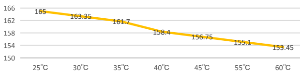
Temperature (Celsius) Derate Curves Unit: kVA
