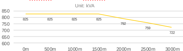
Altitude (meters) Derate Curves
