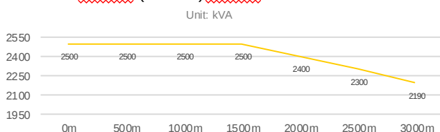
Altitude (meters) Derate Curves
