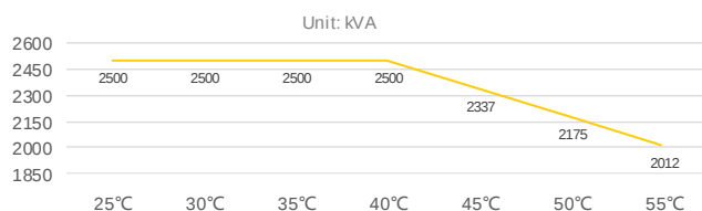
Temperature (Celsius) Derate Curves
