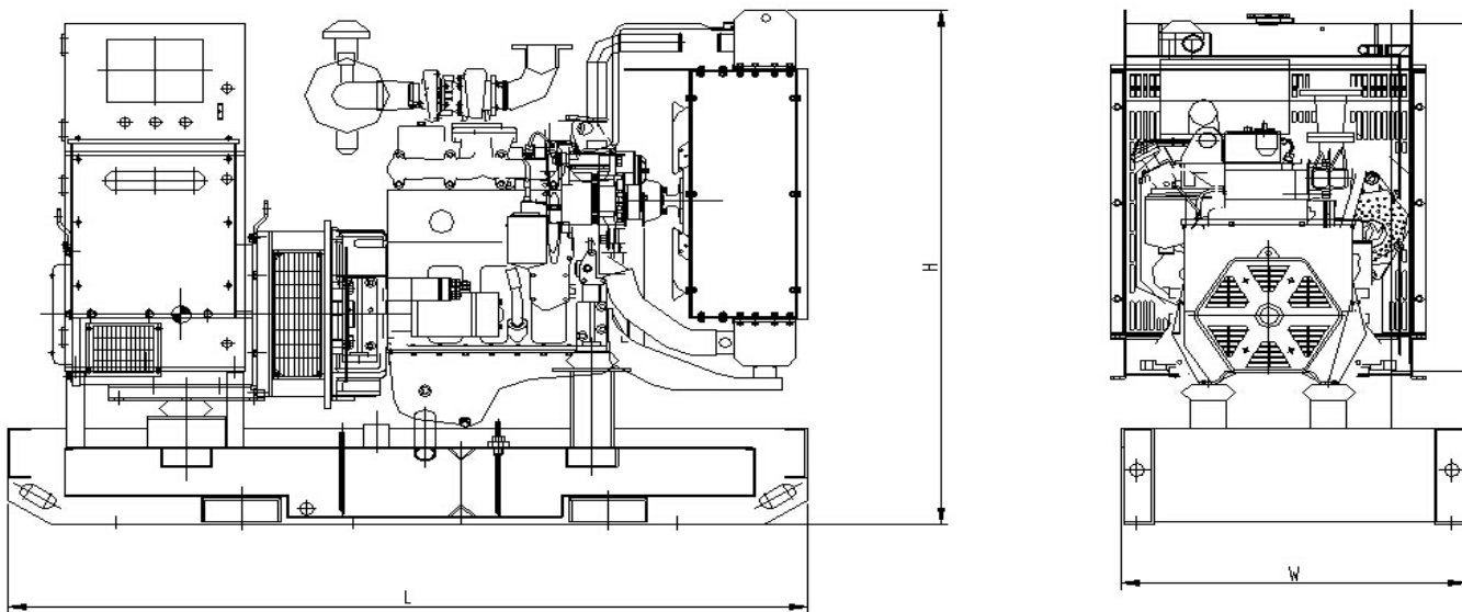
LSP565E3-6 (Open type)
