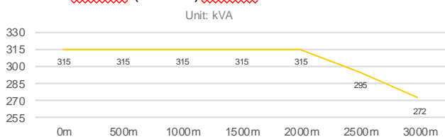
Altitude (meters) Derate Curves
