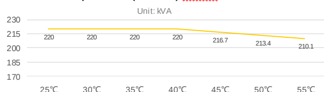
Temperature (Celsius) Derate Curves
