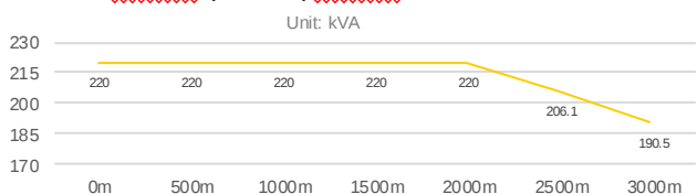
Altitude (meters) Derate Curves
