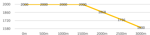
Altitude (meters) Derate Curves
